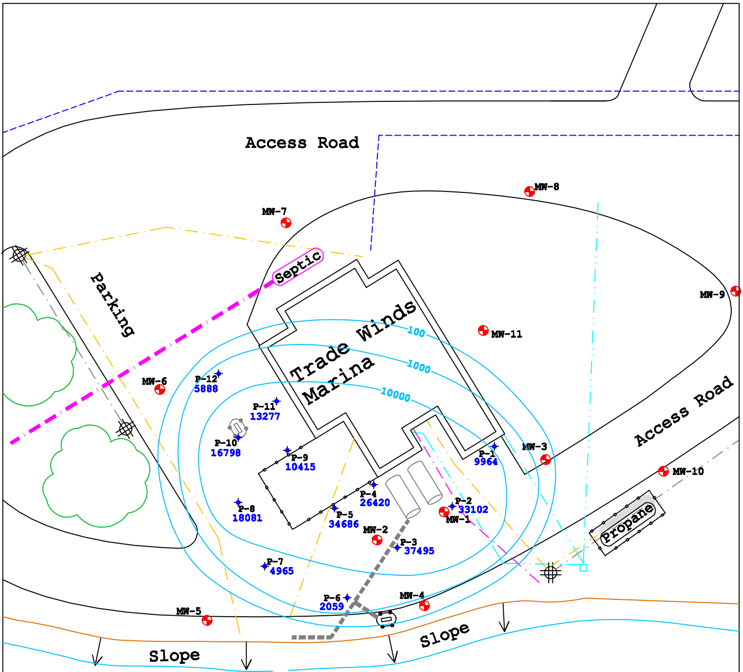
Benzene Isoconcentration Map 16-Foot Depth
