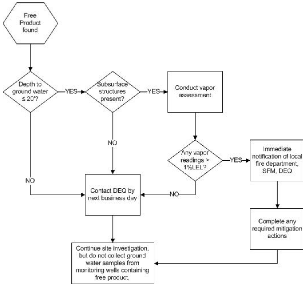
Figure 4-1. Free Product Response Process
