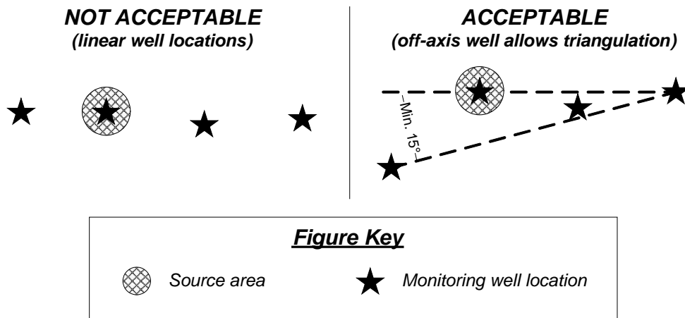
Figure 4-2. Well Placement for Determining Ground Water Flow Direction
